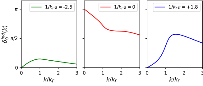
FIG. 4. Induced scattering phase shift \delta_0^{\text{ind}}(k) for the potentials in Fig. 2. The initial slope near k = 0 determines the induced scattering lengths k_F a_{\text{ind}} = -0.8; +0.7; -1.0 from left to right. On the a > 0 side the phase shift steeply rises above \pi/2 indicating a quasi-bound state. Data shown for Cs-Li mass ratio M/m = 22.17 .
